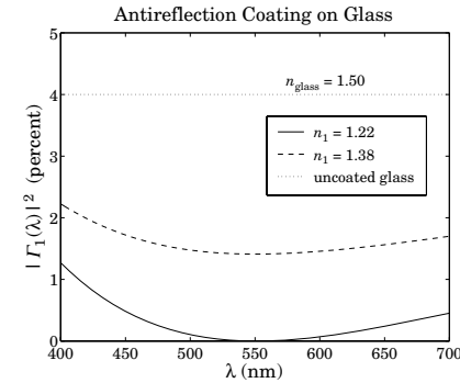
Fig. 5.5.3 Reflectance over the visible spectrum.
