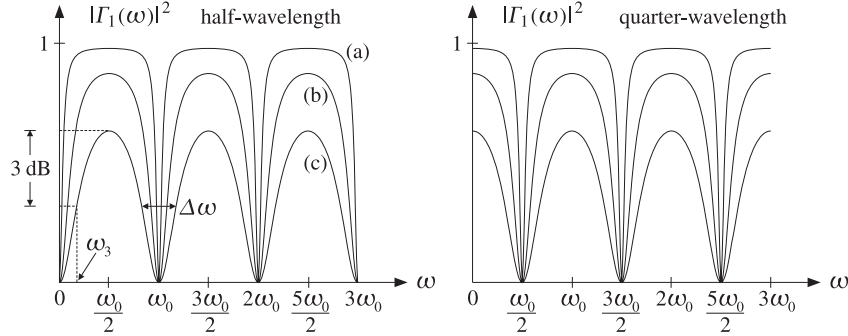
Fig. 5.5.1 Reflection responses |Γ(ω)|^2 . (a) |\rho_1| = 0.9 , (b) |\rho_1| = 0.7 , (c) |\rho_1| = 0.5 .
